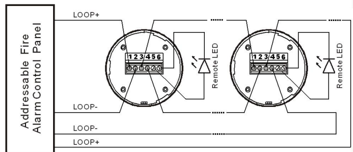
Figure 1. Wiring diagram:
